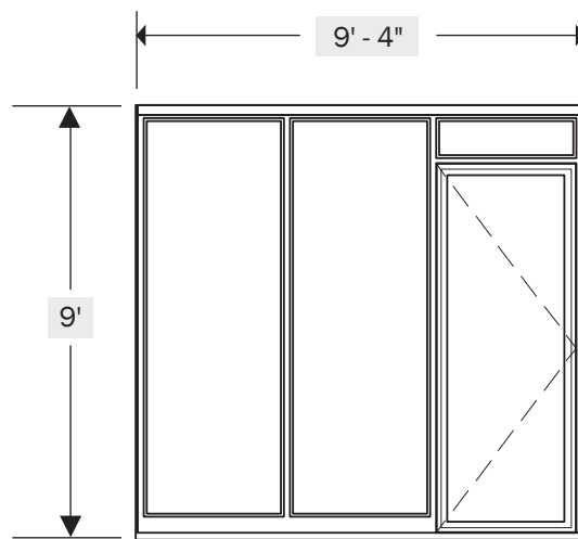
84 SQ. FT. WINDOW ELEVATION AS VIEWED FROM LIVING AREA OF SUITE F
