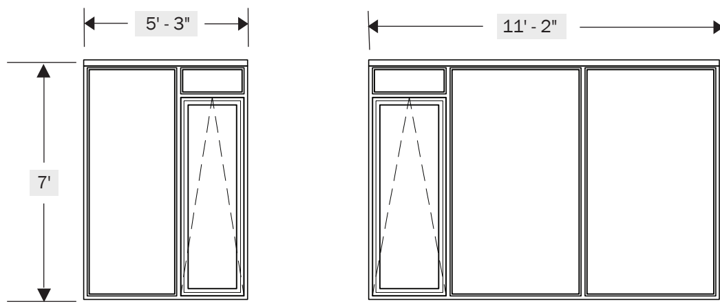
125 SQ. FT. WINDOW ELEVATION AS VIEWED FROM LIVING AREA AND BEDROOM
