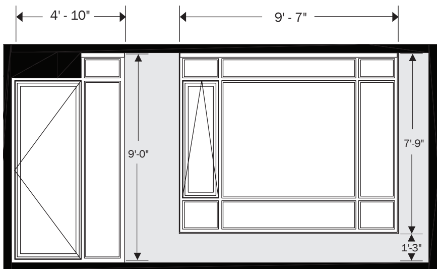
118 SQ. FT. WINDOW ELEVATION AS VIEWED LIVING AREA
