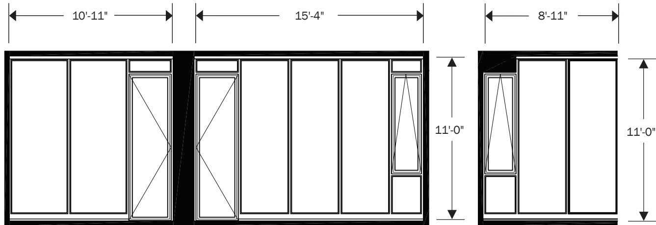
385 SQ. FT. TOTAL WINDOW ELEVATIONS AS VIEWED FROM LIVING ROOM & MASTER BEDROOM
